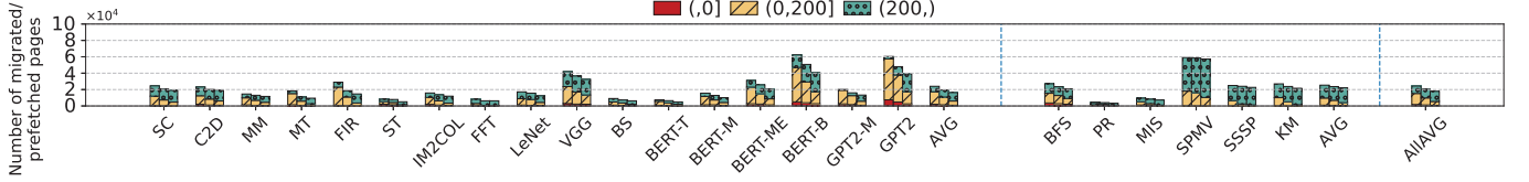
Fig. 20. Total remote access changes for migrated/prefetched pages (left: regular benchmarks, middle: irregular benchmarks, right: overall average). The bars for each benchmark, from left to right, represent LIBRA w/o cost estimation & coordination, LIBRA w/o coordination, and LIBRA
